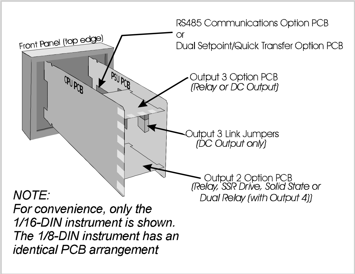
Figure 2-1 PCB Positions
